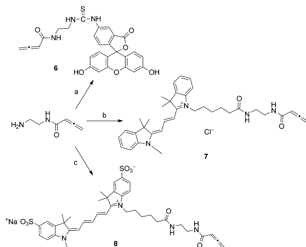
Scheme 3. Synthesis of labeling probes with allenamide handles. Reaction conditions: a) FITC isomer I, DMF, DIPEA, RT, 2 h; b) Cy3-NHS ester, DMF, DIPEA, RT, 2 h; c) sulfo-Cy5-NHS ester, DMF, DIPEA, RT, 2 h. DIPEA = diisopropylethylamine, DMF = N,N -dimethylformamide, FITC = fluorescein isothiocyanate, NHS = N -hydroxysuccinimide.
